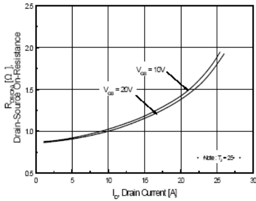
Figure 3. On-Resistance Variation
